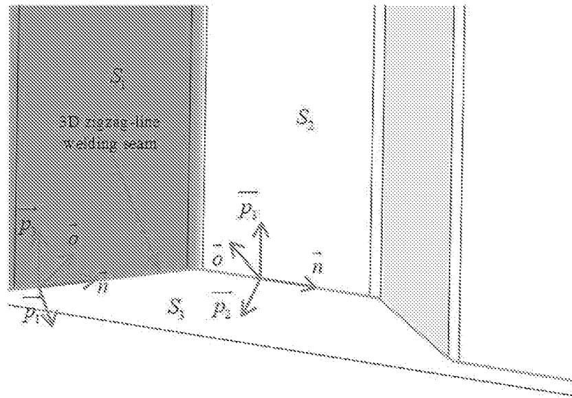
Figure 8. 3D zigzag-line welding seam attitude model.
