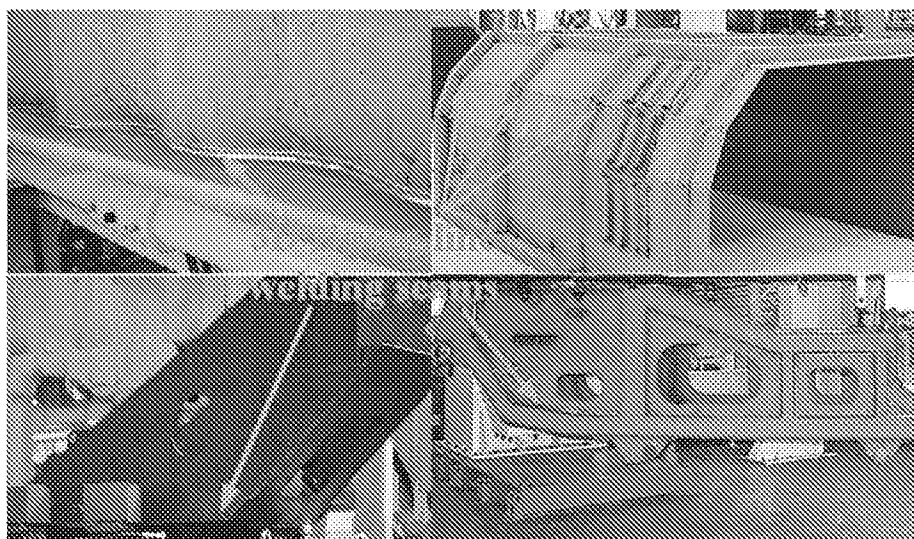
Figure 1. Examples of three-dimensional (3D) zigzag-line welding seams.
