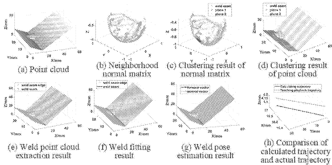
Figure 13. The influence of positioning welding seams on 3D zigzag-line welding seam pose information extraction.
