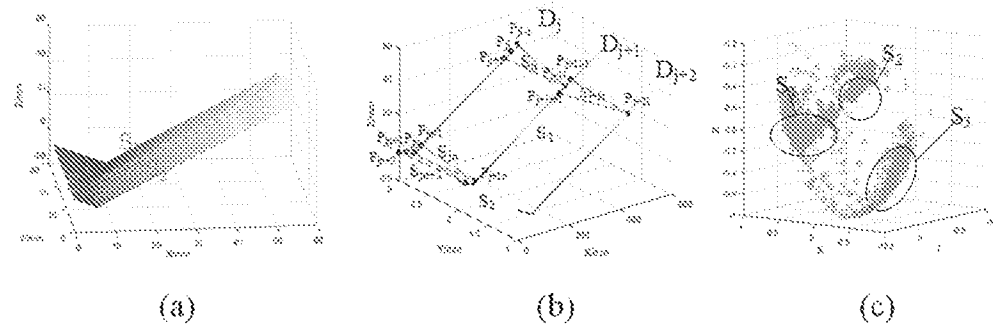
Figure 4. 3D zigzag-line welding seams point cloud data neighborhood normal vectors; (a) Point cloud data; (b) Method for establishing neighborhood normal vectors; (c) Neighborhood normal vectors.
