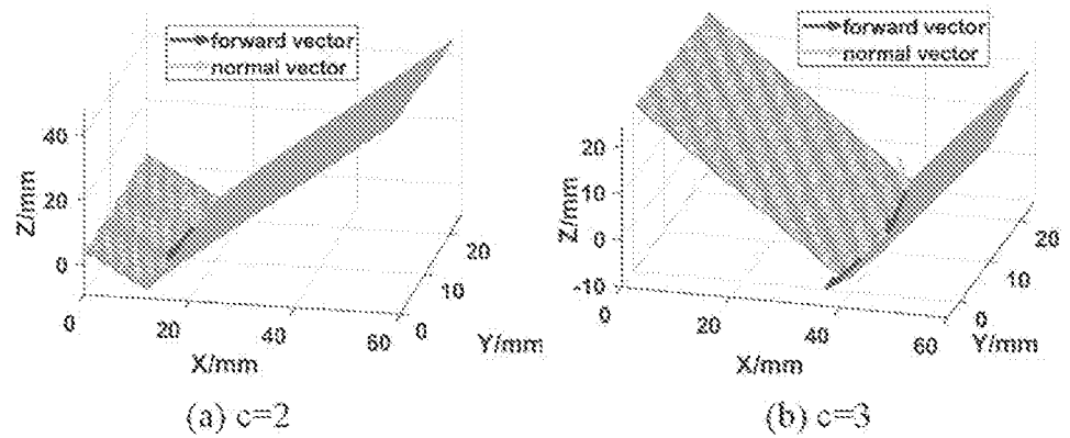
Figure 9. Welding seam attitude estimation results; (a) When c = 2 , the welding seam attitude estimation result; (b) When c = 3 , the welding seam attitude estimation result.
