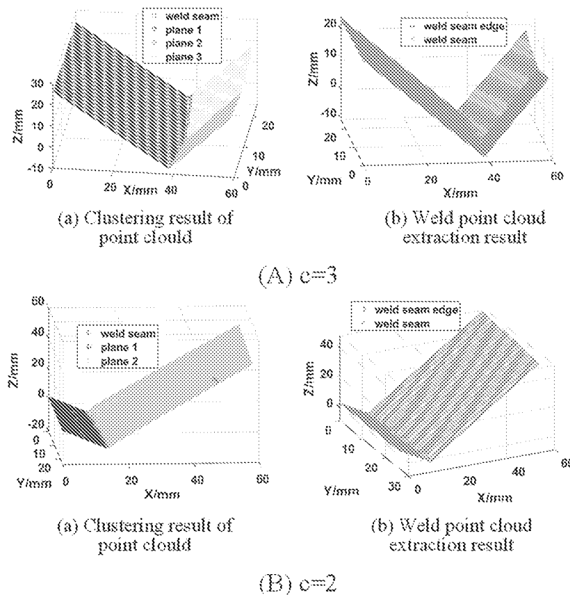
Figure 6. Weld point cloud extraction results.
