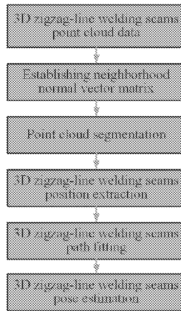
Figure 3. 3D zigzag-line welding seams pose information online fast extraction process.
