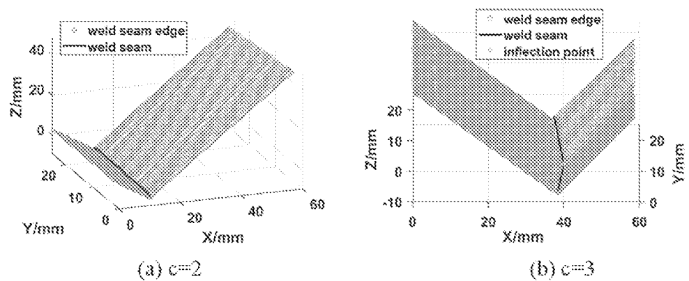
Figure 7. Welding seam trajectory fitting results; (a) When c = 2 , the welding seam trajectory fitting result; (b) When c = 3 , the welding seam trajectory fitting result.
