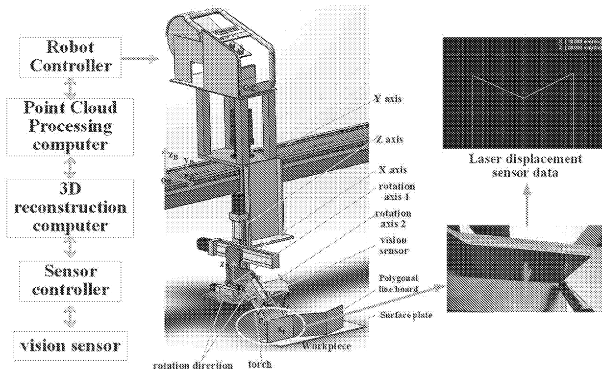
Figure 10. The structure of the experimental system.
