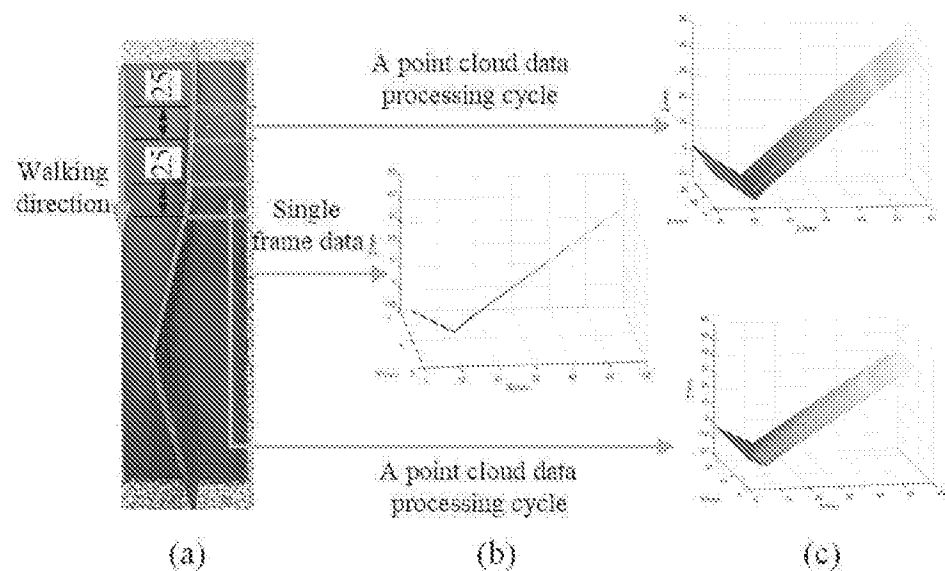
Figure 2. 3D zigzag-line welding seam point cloud data; (a) Workpiece; (b) Single frame data; (c) Point cloud data.
