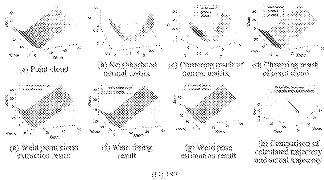
Figure 12. 3D zigzag-line welding seam pose information online extraction results.
