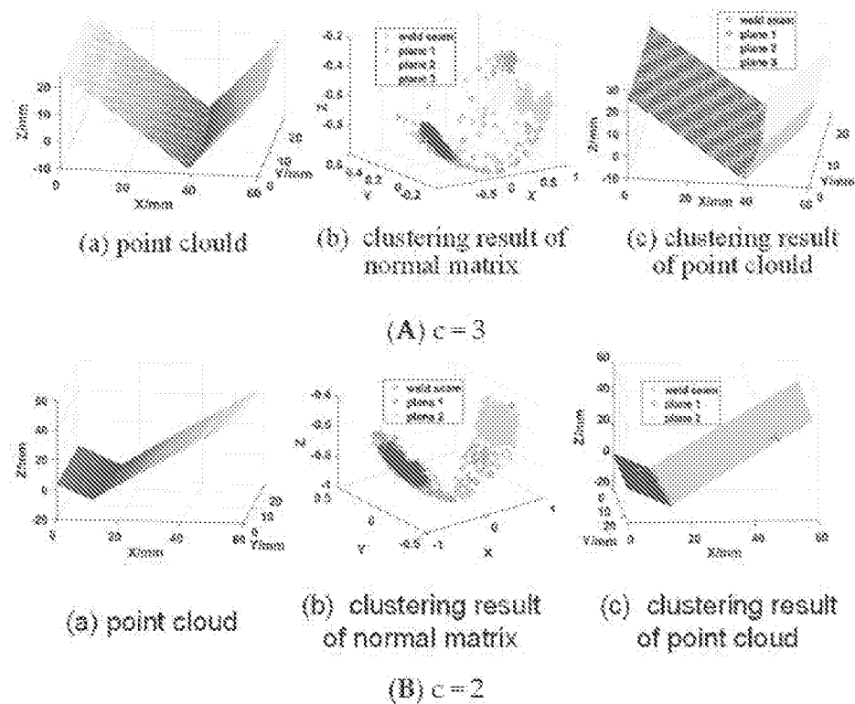
Figure 5. Point cloud segmentation results.
